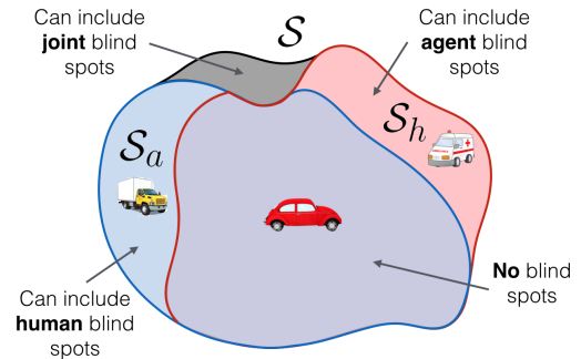
Figure 1: The agent is trained in a simulator world, which sees a subset S_a of the true state space S . Human demonstrations operate in subset S_h , and joint execution happens in the real world space S .
